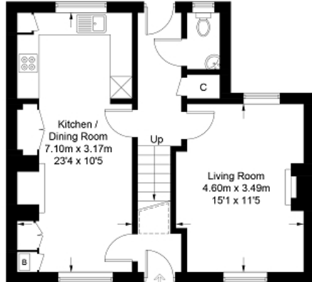
Ground Floor 50.2 sq m / 540 sq ft
